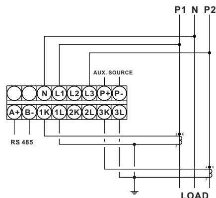
1-Phase 3-Wire(2CTs)
