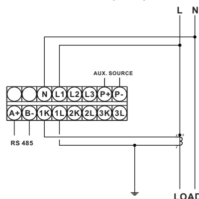
1-Phase 2-Wire(1CT)
