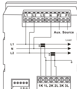
1 Phase 3 Wire(Only 2 CTs)
