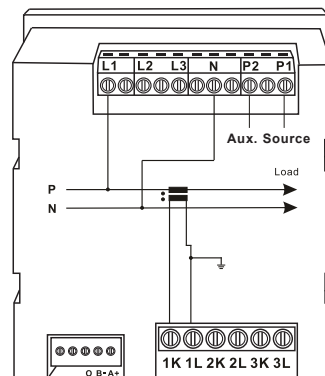
1 Phase 2 Wire(Only 1 CT)
